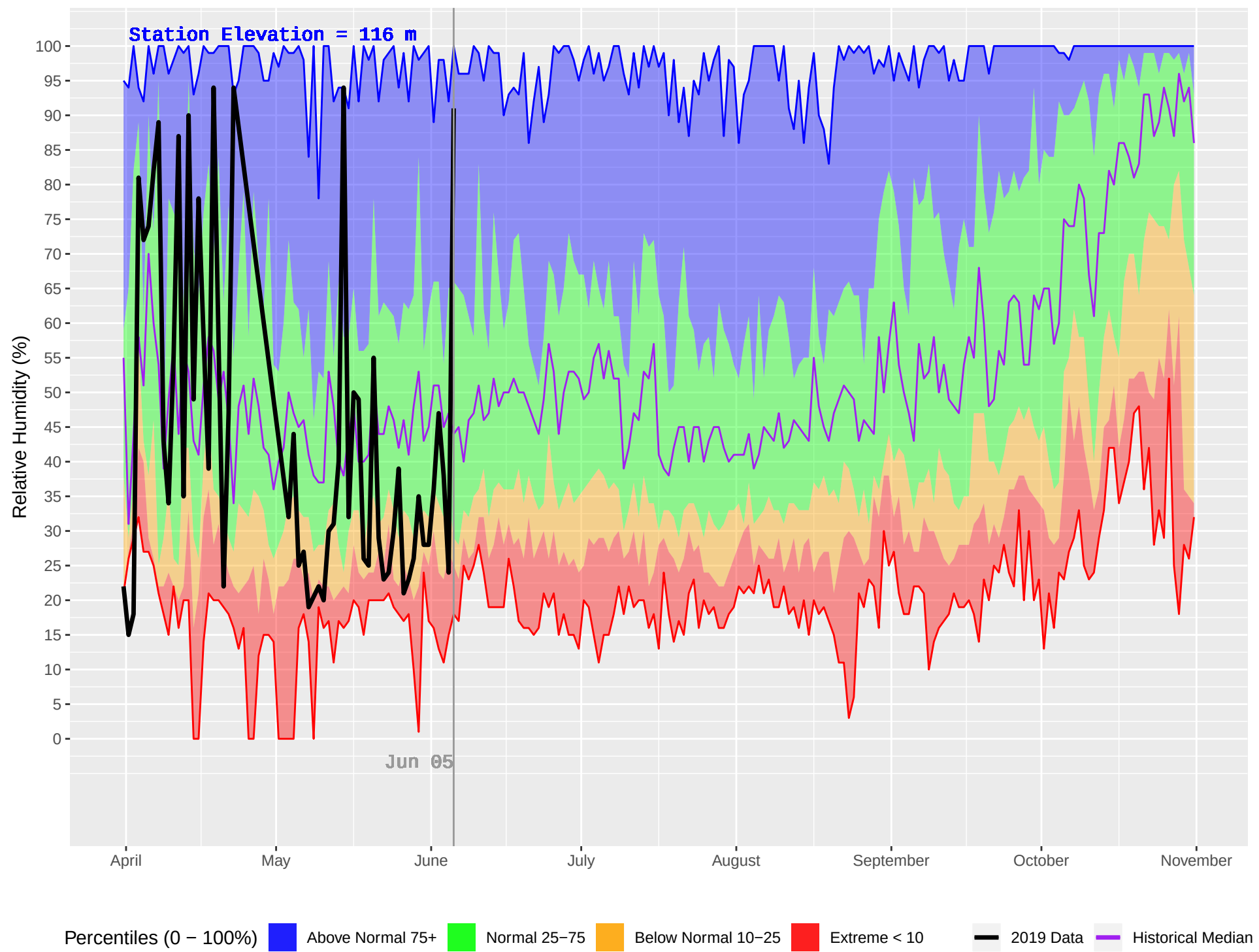
SCAR CREEK (82) : Historical (1982–2018) and Current (2019) Daily Relative Humidity
