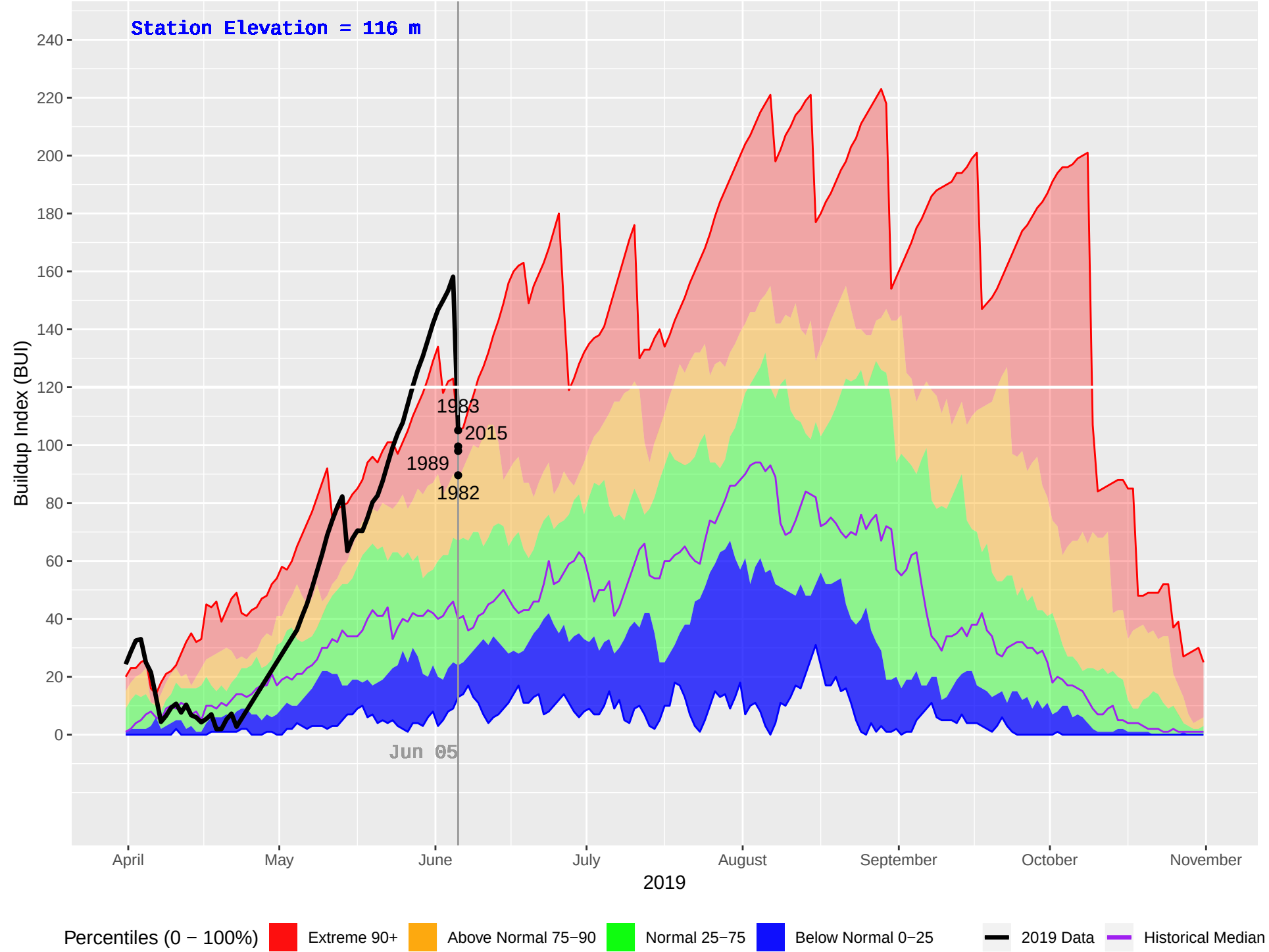
SCAR CREEK (82) : Historical (1982–2018), Current (2019) Daily Buildup Index (BUI)
