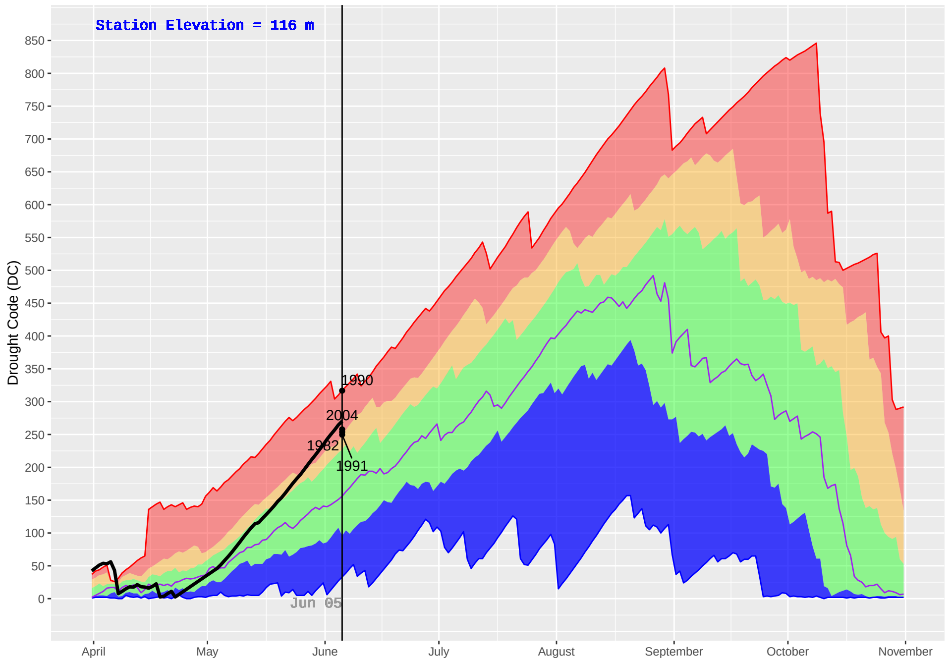
SCAR CREEK (82) : Historical (1982–2018) and Current (2019) Daily Drought Code (DC)
