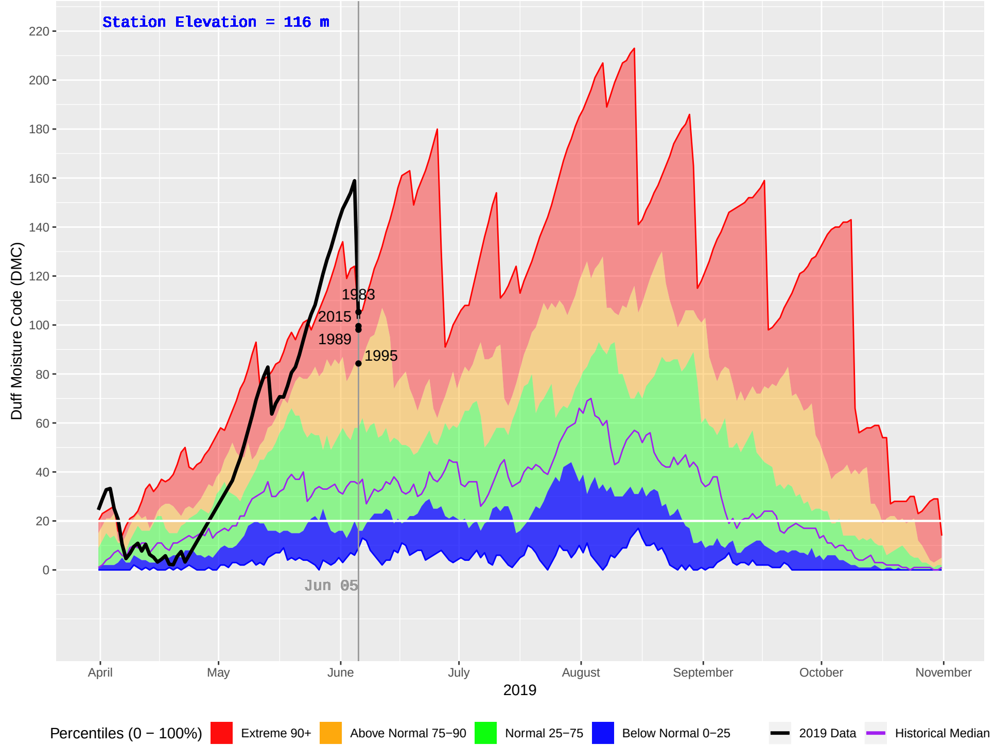
SCAR CREEK (82) : Historical (1982–2018), Current (2019) Daily Duff Moisture Code (DMC)
