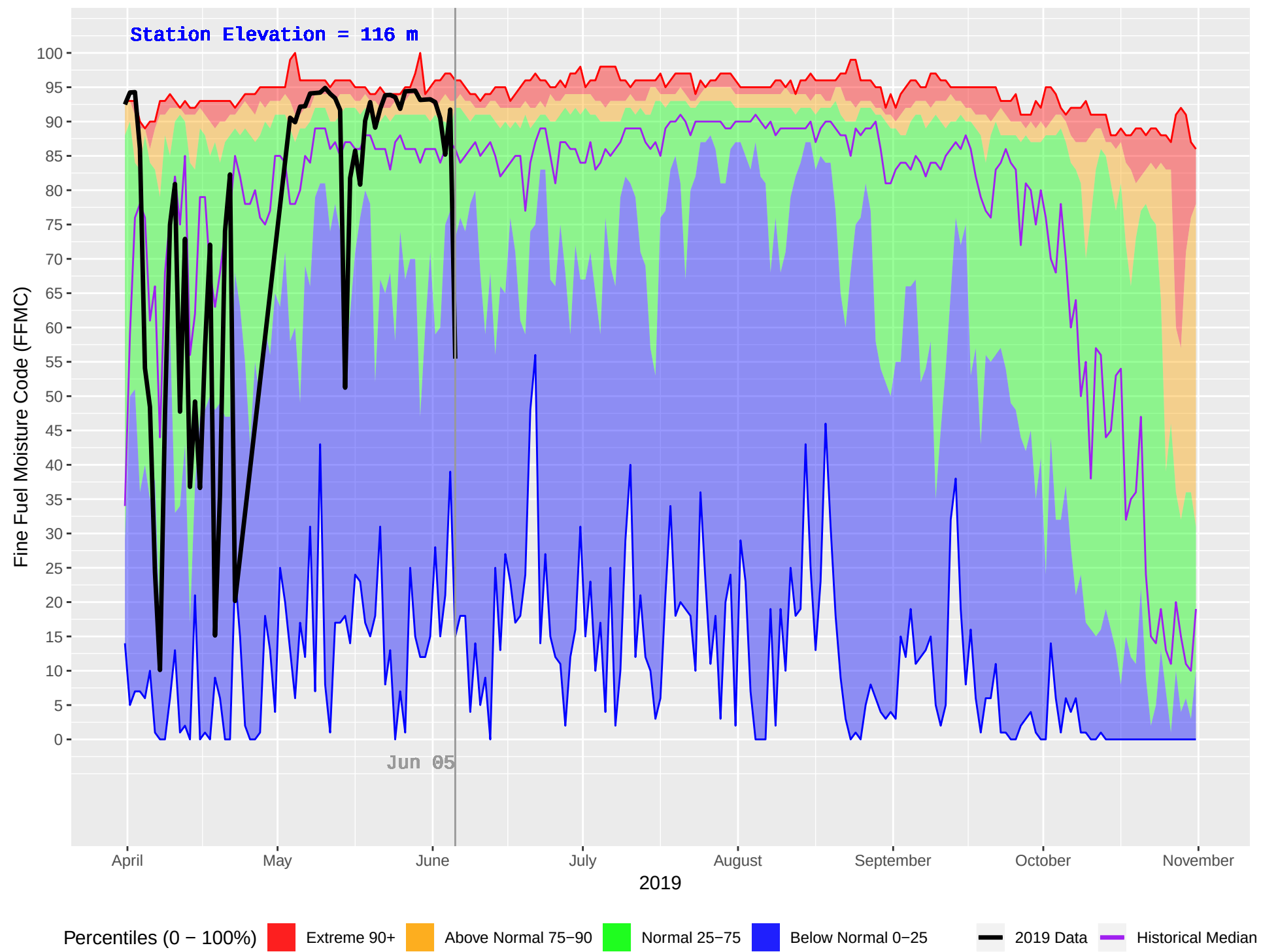
SCAR CREEK (82) : Historical (1982–2018) and Current (2019) Daily Fine Fuel Moisture Code (FFMC)
